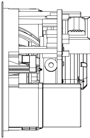
Baffle Side 7.14" (181.1mm)
